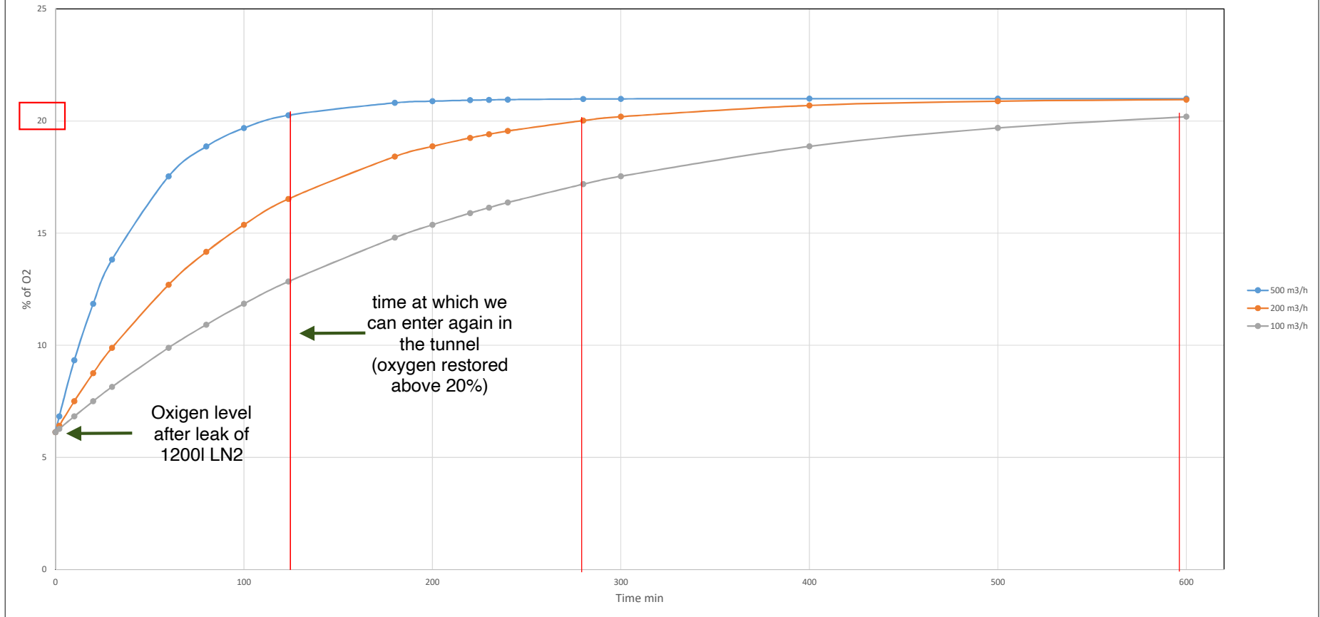
Variation of the Oxygen level in the linac in the case of 1,200 liters of LN2 released in the linac (343 m 3 ) and for three values of fresh air flow rate
